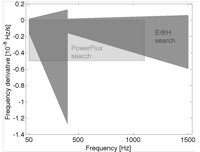
FIG. 7: Comparison of search parameter spaces in the plane of frequency and frequency derivative. The dark-gray region refers to this Einstein@Home all-sky analysis in early LIGO S5 data. The light-grey area corresponds to the recent all-sky PowerFlux search [15] in early LIGO S5 data.
