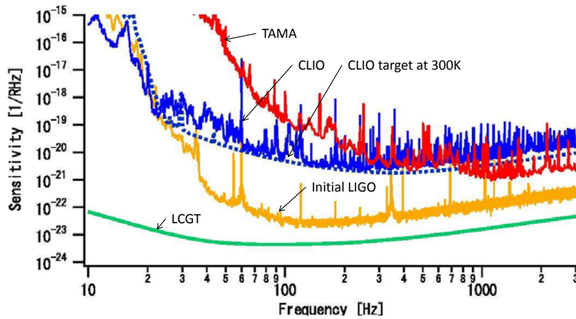
Figure 5. LCGT sensitivity compared with those of CLIO (October 2008, room temperature), CLIO (target, room temperature), TAMA, LIGO (Science run 5). The horizontal axis is frequency [Hz] and the vertical axis represents the sensitivity spectrum for gravitational waves [ 1/\sqrt{\text{Hz}} ]. Notwithstanding the short baseline length of CLIO, sensitivity comparable to that of LIGO at low frequencies clearly shows the merit of the underground location.
