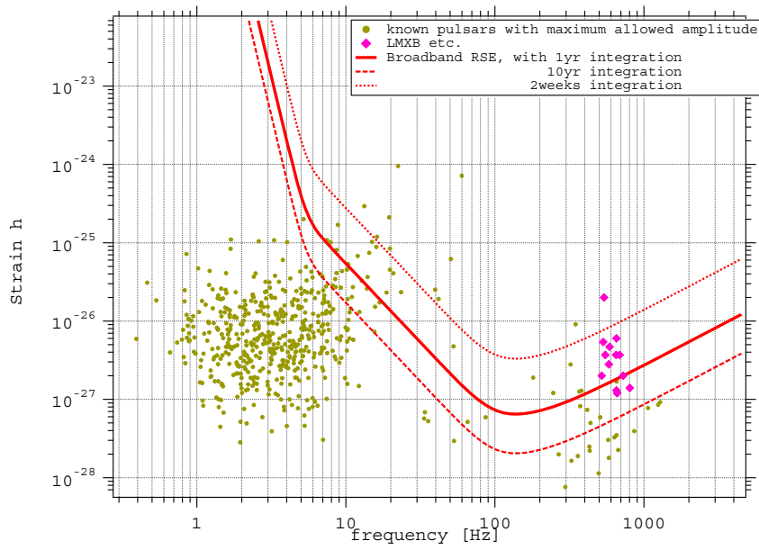
Figure 2. Expected continuous wave sources of a pulsar according to the default design. Circular dots represent the known pulsars with maximum allowed amplitudes, and diamond symbol represents the possible waves from low mass X-ray binaries.
