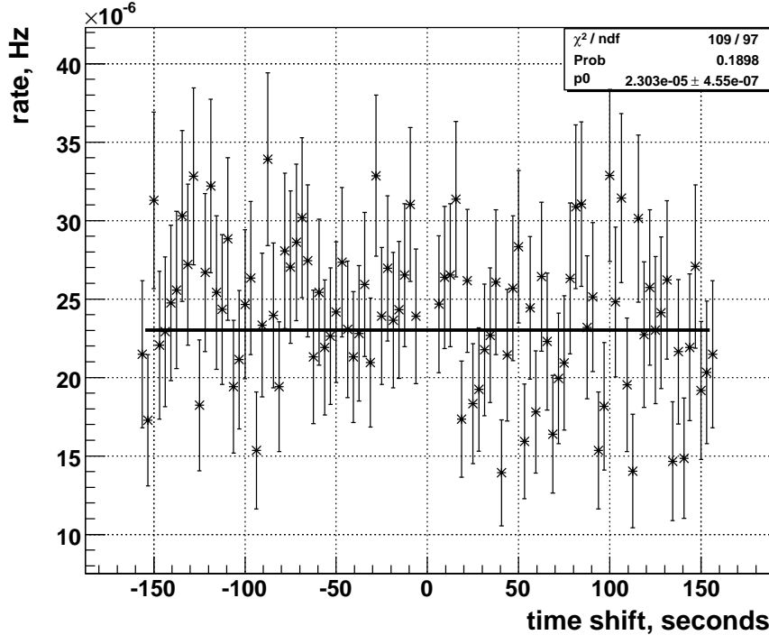
Figure 4. WaveBurst trigger rate as a function of the relative time shift applied between the Hanford and Livingston data streams. The horizontal line is a fit to a constant value.
