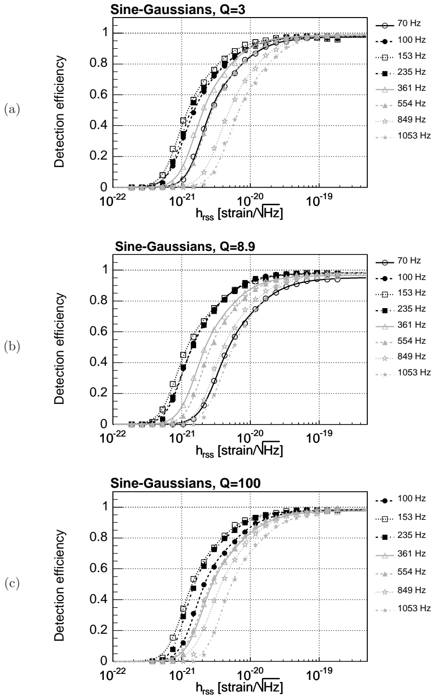
Figure 9. Efficiency curves for simulated gravitational-wave signals: linearly-polarized sine-Gaussian waves with (a) Q=3 ; (b) Q=8.9 ; (c) Q=100 . Statistical errors are comparable to the size of the plot symbols.
