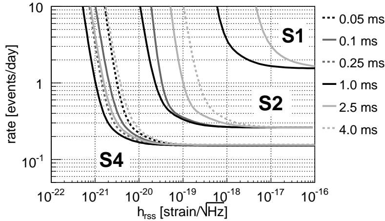
(b) Gaussians
