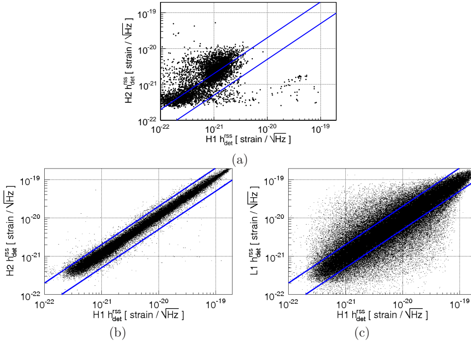
Figure 5. (a) Scatter plot of H2 vs. H1 amplitudes reconstructed by WaveBurst for the tuning set of time-shifted triggers. (b) Scatter plot of H2 vs. H1 amplitudes reconstructed for simulated sine-Gaussian signals with a wide range of frequencies and amplitudes from sources uniformly distributed over the sky (see section 7). In these plots, the diagonal lines show the limits of the H1/H2 amplitude consistency cut: 0.5 < \text{ratio} < 2 . (c) Scatter plot of L1 vs. H1 amplitudes for the same simulated sine-Gaussian signals. Diagonal lines are drawn at ratios of 0.5 and 2 only to guide the eye; no cut is applied using this pair of interferometers.
