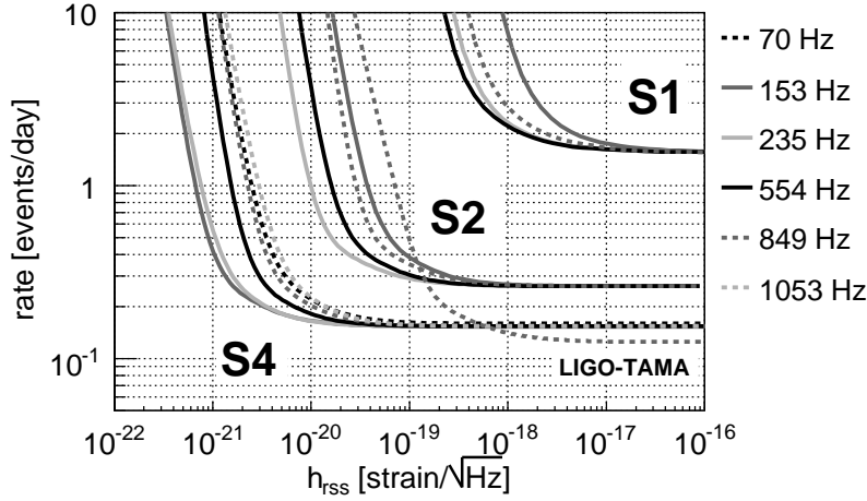
(a) Sine-Gaussians with Q=8.9
