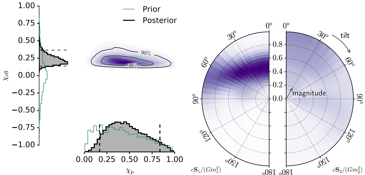
FIG. 4. Left : Posterior density function for the \chi_p and \chi_{\text{eff}} spin parameters (measured at 20 Hz) compared to their prior distributions. The 1-dimensional plot shows probability contours of the prior (green) and marginalized posterior density function (black) [60, 61]. The 2-dimensional plot shows the contours of the 50% and 90% credible regions plotted over a color-coded posterior density function. The dashed lines mark the 90% credible interval. Right : Posterior density function for the dimensionless component spins, cS_1/(Gm_1^2) and cS_2/(Gm_2^2) , relative to the normal of the orbital plane \hat{\mathbf{L}} . S_i and m_i are the spin angular momenta and masses of the primary ( i = 1 ) and secondary ( i = 2 ) black holes, c is the speed of light and G is the gravitational constant. The posterior density functions are marginalized over the azimuthal angles. The bins are designed to have equal prior probability; they are constructed linearly in spin magnitudes and the cosine of the tilt angles \cos^{-1}(\hat{\mathbf{S}}_i \cdot \hat{\mathbf{L}}) .
