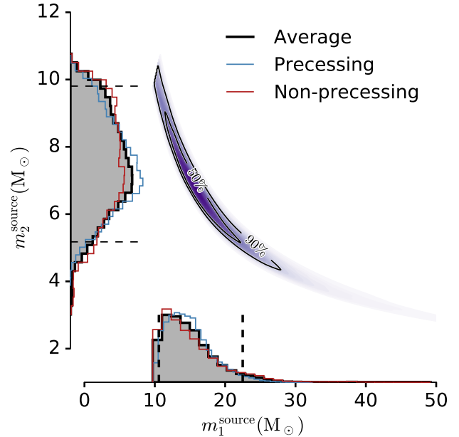
FIG. 3. Posterior density function for the source-frame masses m_1^{\text{source}} (primary) and m_2^{\text{source}} (secondary). The 1-dimensional marginalized distributions include the posterior density functions for the precessing (blue) and non-precessing (red) spin waveform models where average (black) represents the mean of the two models. The dashed lines mark the 90% credible interval for the average posterior density function. The 2-dimensional plot shows the contours of the 50% and 90% credible regions plotted over a color-coded posterior density function.
