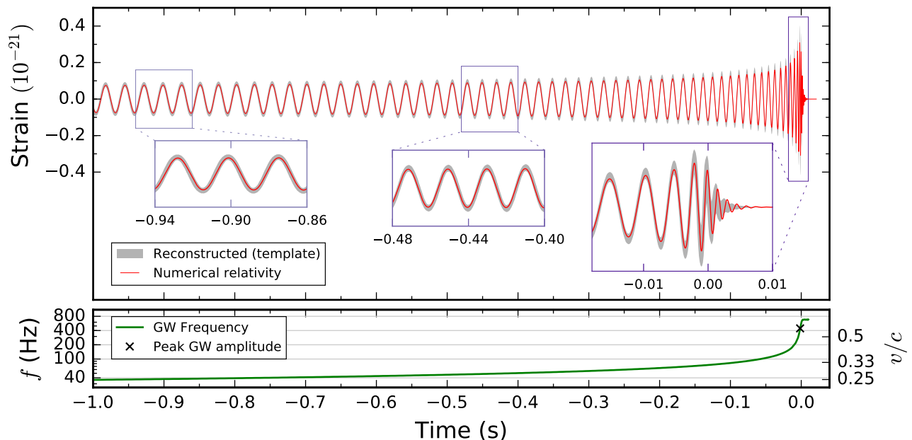
FIG. 5. Estimated gravitational-wave strain from GW151226 projected onto the LIGO Livingston detector with times relative to December 26, 2015 at 03:38:53.648 UTC. This shows the full bandwidth, without the filtering used for Fig. 1. Top : The 90% credible region (as in [59]) for a non-precessing spin waveform-model reconstruction (grey) and a direct, non-precessing numerical solution of Einstein’s equations (red) with parameters consistent with the 90% credible region. Bottom : The gravitational-wave frequency f (left axis) computed from the numerical-relativity waveform. The cross denotes the location of the maximum of the waveform amplitude, approximately coincident with the merger of the two black holes. During the inspiral, f can be related to an effective relative velocity (right axis) given by the post-Newtonian parameter v/c = (GM\pi f/c^3)^{1/3} , where M is the total mass.
