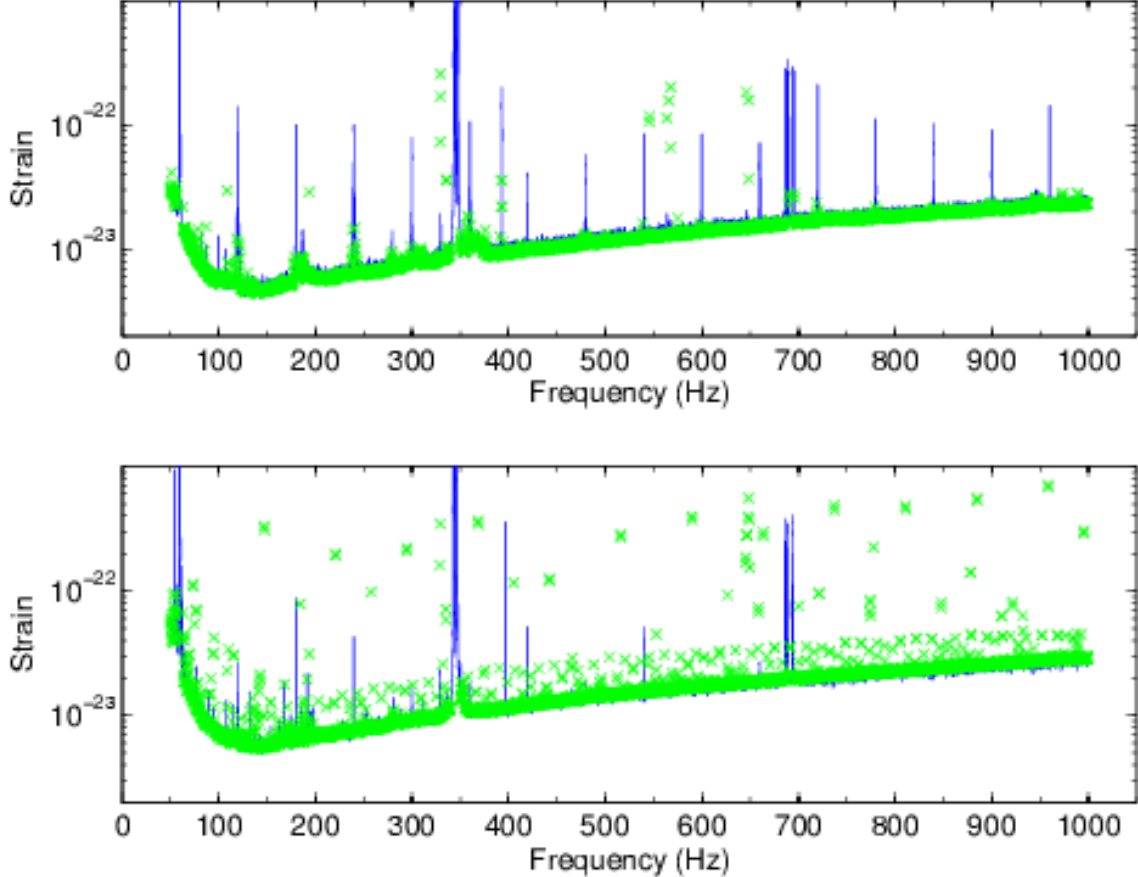
FIG. 27: The solid curve shows the characteristic amplitude given by Eq. (B11) and crosses show the measured upper limits on h_0 for the StackSlide search of the H1 (top) and L1 (bottom) data.
