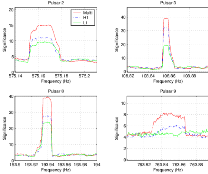
FIG. 17: Maximum significance as a function of frequency corresponding to the multi-interferometer search (using the data from the three detectors) and the H1 and L1 alone.
