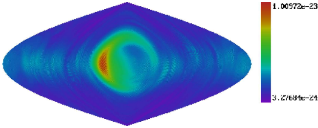
FIG. 22: Sample sky map of Feldman Cousins upper limits on circularly polarized strain for a 0.25-Hz band containing hardware-injected Pulsar 2 at 575.16 Hz. Only the data (half the run) during which the pulsar injection was enabled has been analyzed for this plot. The injected pulsar ( h_0 = 8.0 \times 10^{-24} ) stands out clearly above background. (Right ascension increases positively toward the left and declination toward the top of the sky map.)
