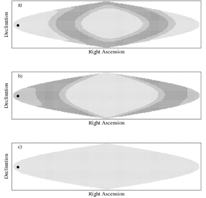
FIG. 13: S4 sky band regions (good - light gray, bad for L1 - medium or dark gray, bad for H1 & L1 - dark gray) for a source frequency \hat{f} = 300 Hz and three different assumed spin-down choices: a) zero; b) -3 \times 10^{-9} Hz s ^{-1} ; and c) -1 \times 10^{-8} Hz s ^{-1} . The black circle indicates the average position of the Sun during the data run.
