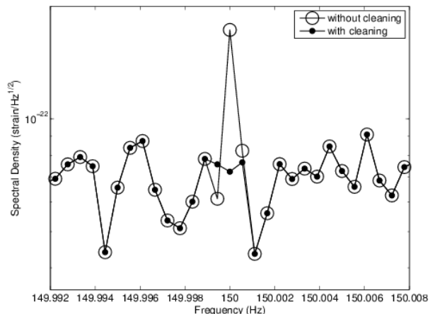
FIG. 5: The L1 amplitude spectral density in a narrow frequency band estimated from 10 SFTs before and after the line cleaning used by the StackSlide pipeline. In the band shown, the 150 Hz bin, and one bin either side of this bin have been replaced with estimates of the noise based on neighboring bins.
