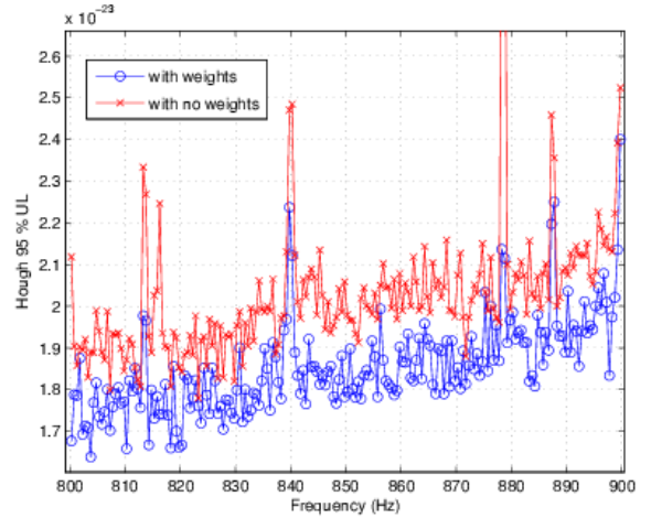
FIG. 34: Comparison of the upper limits obtained using 500 Monte Carlo injections with and without weights in 0.5 Hz bands for the Hough multi-interferometer search. The use of the weights improves the upper limits by a \sim 9\% factor.
