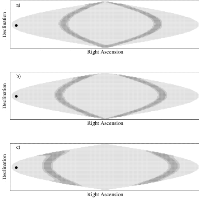
FIG. 14: S4 sky band regions (good - light gray, bad for L1 - medium or dark gray, bad for H1 & L1 - dark gray) for a source frequency \hat{f} = 1000 Hz and three different assumed spin-down choices: a) zero; b) -3 \times 10^{-9} Hz s ^{-1} ; and c) -1 \times 10^{-8} Hz s ^{-1} . The black circle indicates the average position of the Sun during the data run.
