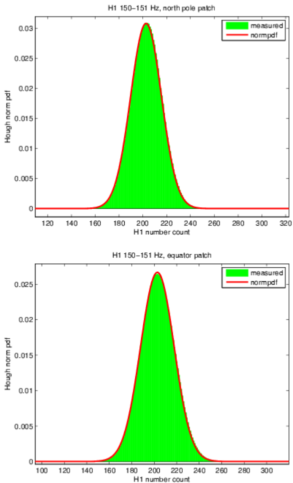
FIG. 8: Two example histograms of the normalized Hough number count compared to a Gaussian distribution for the H1 detector in the frequency band 150-151 Hz. The upper figure corresponds to a patch located at the north pole for the case in which the weights are used. The number of templates analyzed in this 1Hz band is of 11 \times 10^6 , the number of SFTs 1004, the corresponding mean \bar{n} = 202.7 and \sigma = 12.94 is obtained from the weights. The lower figure corresponds to a patch at the equator using the same data. In this case the number of templates analyzed in this 1Hz band is of 10.5 \times 10^6 , and its corresponding \sigma = 14.96 .
