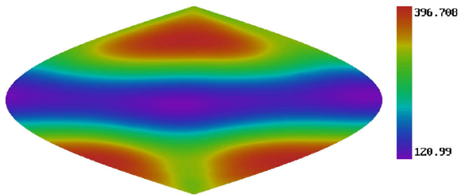
FIG. 11: Sky map of run-summed PowerFlux weights for a 0.25-Hz band near 575 Hz for one choice of linear polarization in the S4 H1 data. The normalization corresponds roughly to the effective number of median-noise SFT’s contributing to the sum.
