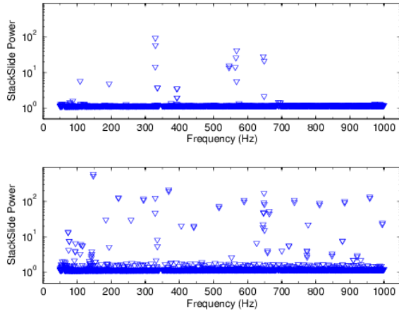
FIG. 23: The loudest observed StackSlide Power for H1 (top) and L1 (bottom). Frequency bands with the harmonics of 60 Hz and the violin modes have been removed.
