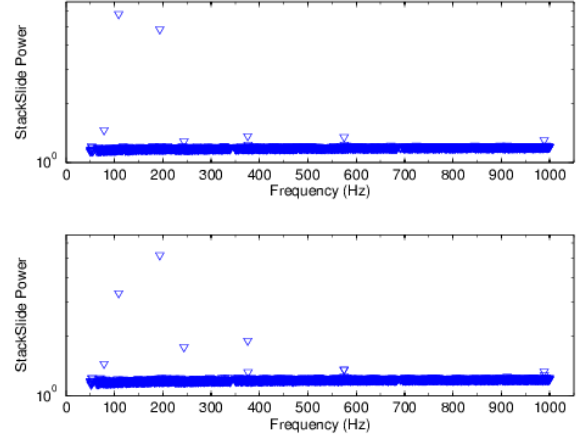
FIG. 24: The loudest observed StackSlide Power for H1 (top) and L1 (bottom) with a simple veto applied: only outliers in each 0.25 Hz band with SNR > 7 in both interferometers that have a fractional frequency difference \leq 2.2 \times 10^{-4} are kept. These are shown against the background results that have SNR \leq 7 in both interferometers. Frequency bands with the harmonics of the 60 Hz and the violin modes have also been removed.
