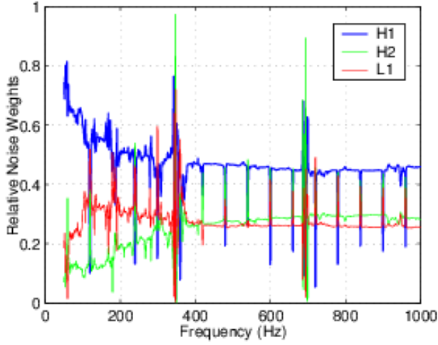
FIG. 28: Relative contributions of the three interferometers in the Hough multi-interferometer search. The noise weights are calculated in 1 Hz bands.
