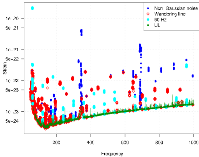
FIG. 36: PowerFlux limits on linearly polarized CW radiation amplitude for the L1 data from the S4 run, with the same color coding as in the preceding figure.
