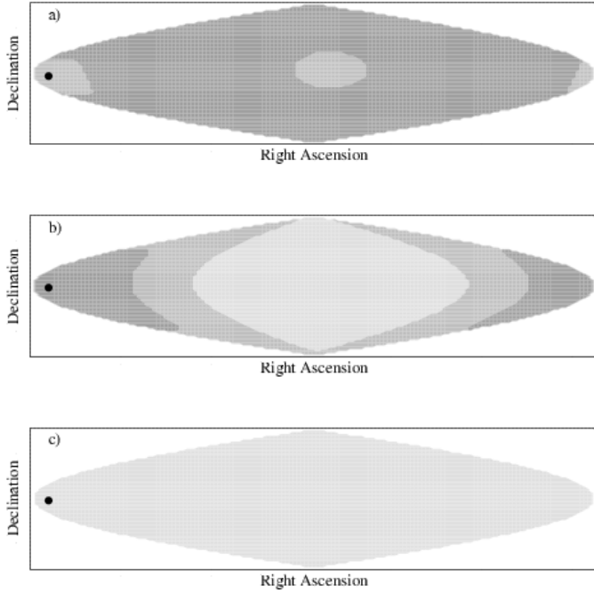
FIG. 12: S4 sky band regions (good - light gray, bad for L1 - medium or dark gray, bad for H1 & L1 - dark gray) for a source frequency \hat{f} = 100 Hz and three different assumed spin-down choices: a) zero; b) -3 \times 10^{-9} Hz s ^{-1} ; and c) -1 \times 10^{-8} Hz s ^{-1} . The black circle indicates the average position of the Sun during the data run.
