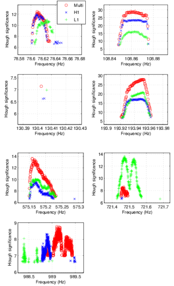
FIG. 30: Hough significance of the outliers that have survived the coincidence analysis without considering the bands contaminated with 60 Hz harmonics or the violin modes. Points are plotted only for multi-interferometer templates with significance greater than 7 and for single-interferometer templates with significance greater than 6.6.
