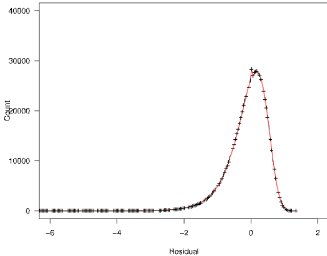
FIG. 10: Typical residual logarithmic power following noise decomposition for a sample 0.25-Hz band of H1 data (crosses) near 575 Hz in a band containing an injected pulsar. The residual is defined as the difference between a measured power for a given frequency bin in a given 30-minute period and the value predicted by the FMedians and TMedians vectors. The smooth curve is for a simulation in Gaussian noise.
