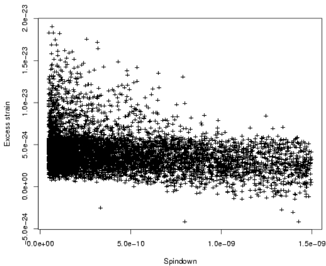
FIG. 20: “Excess” (upper limit minus injected) strain plotted vs injected signal spin-down for sample PowerFlux H1 elliptic-polarization near 140 Hz injections.
