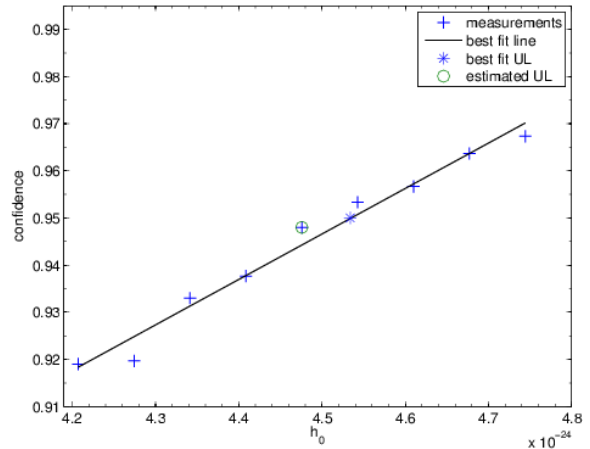
FIG. 6: Measure confidence vs. h_0 for an example band (140–140.25 Hz in H1). A best-fit straight line is used to find the value of h_0 corresponding to 95% confidence and to estimate the uncertainties in the results (see text).
