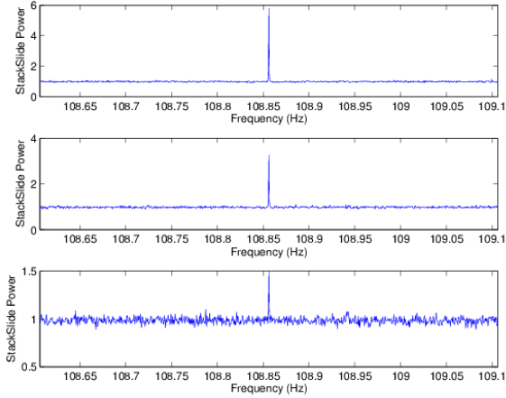
FIG. 25: The StackSlide Power vs. frequency for H1 (top), L1 (middle) and H2 (bottom) using the sky position and the \dot{f} value of the template that gives the outlier in H1, for outlier number 2 given in Table IX. Comparing with Tables V and VI this outlier is identified as due to hardware injection Pulsar3.
