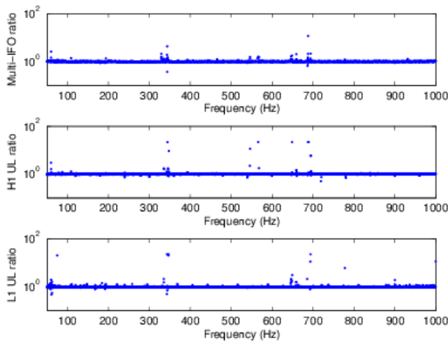
FIG. 33: Ratio of the 95% confidence all-sky upper limits on h_0 obtained from the Hough search by means of Monte Carlo injections to those predicted by Eq. (44) of the multi-interferometer (top), H1 (middle) and L1 (bottom) data. The comparison is performed in 0.25 Hz bands. The scale factors C used are 11.0 for the multi-interferometer search, 11.5 for H1 and 11.1 for L1.
