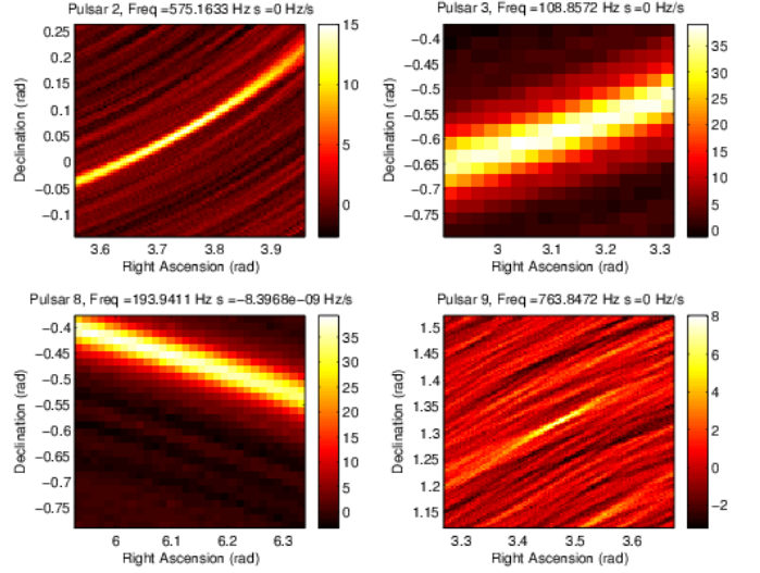
FIG. 18: Maps of the Hough significance corresponding to the multi-interferometer case for Pulsar2, Pulsar3, Pulsar8 and Pulsar9. The location of the injected pulsars are the centers of the maps. For Pulsar2, Pulsar3 and Pulsar9, the maps correspond to the frequency and spin-down values closest to the real injected ones. For Pulsar8, we show the map containing the maximum significance value. The discrepancy in sky location is due to the mismatch in frequency and spin-down values between those used in the injections and those corresponding to the Hough map.
