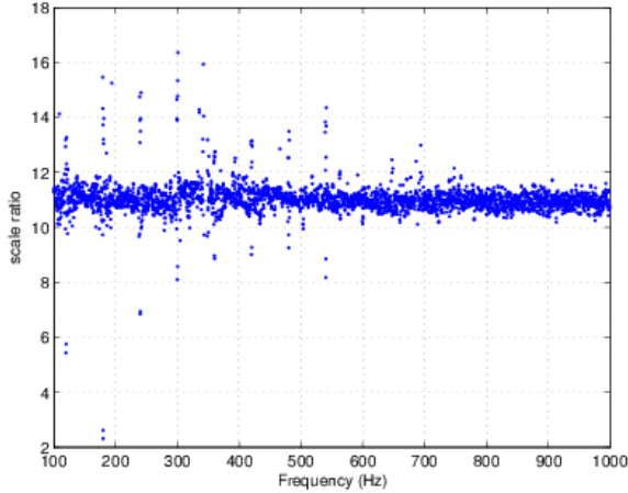
FIG. 32: Ratio of the upper limits measured by means of Monte-Carlo injections in the multi-interferometer Hough search to the quantity h_0^{95\%}/C as defined in Equation (44). The value of \mathcal{S} in equation (44) is computed using the false alarm \alpha_H corresponding to the observed loudest event, in a given frequency band, and for a false dismissal rate \beta_H = 0.05 , in correspondence to the desired confidence level of the upper limit. The comparison is performed in each 0.25 Hz band. Analysis of the full bandwidth, and also in different 100 Hz bands, yield a scale factor C to be 11.0 \pm 0.5 .
