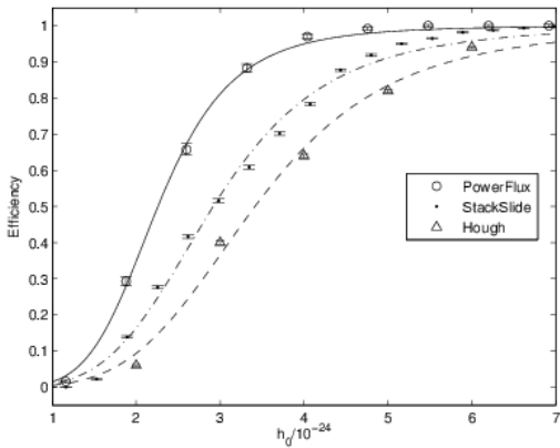
FIG. 39: Comparison of StackSlide, Hough, and PowerFlux efficiencies (SNR > 7 ) vs injected strain amplitude h_0 for the band 140.50-140.75 Hz for H1. From left to right, the curves correspond to PowerFlux, StackSlide, and Hough. This band is typical of those without large outliers.
