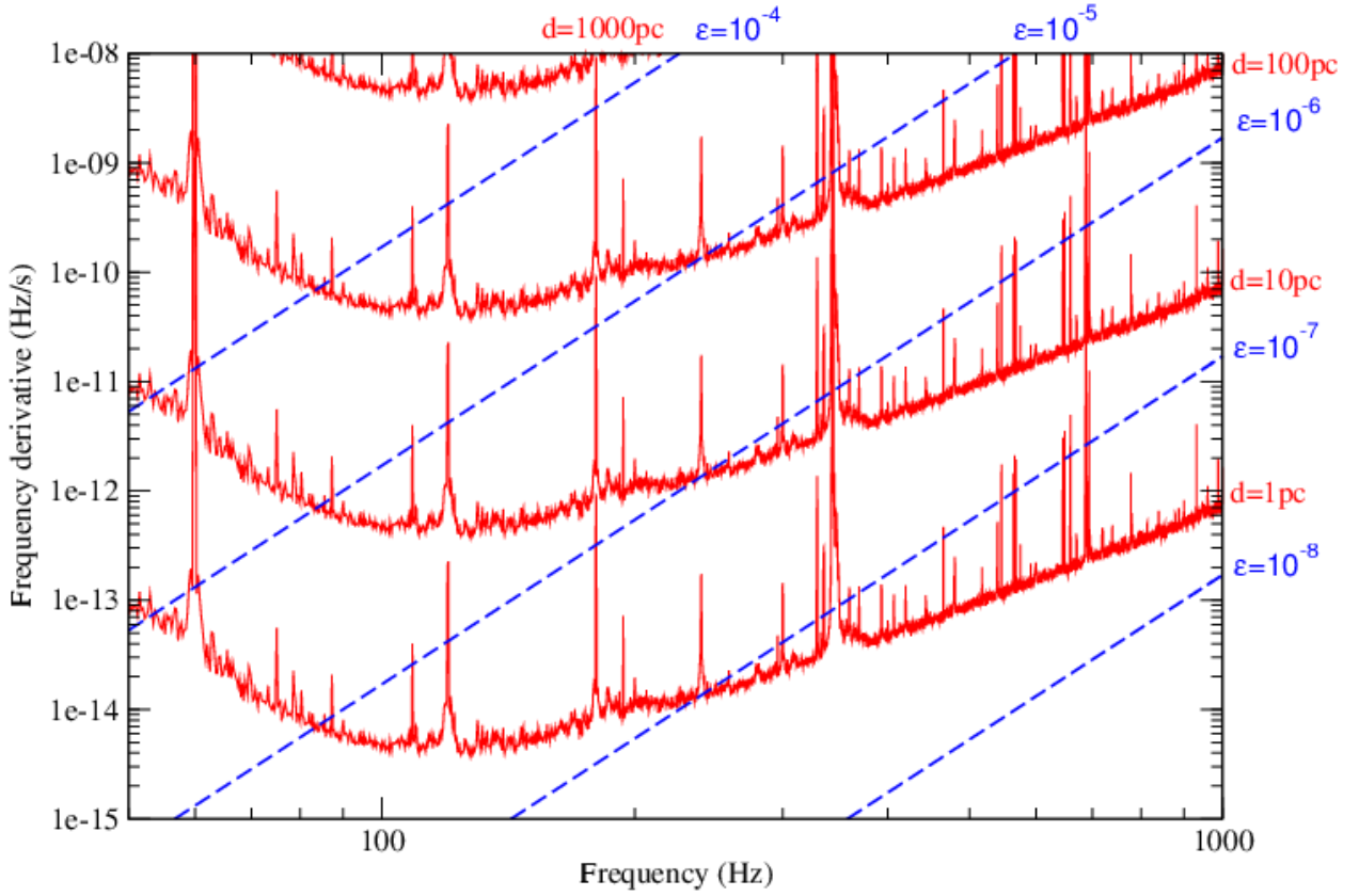
FIG. 41: Range of the multi-interferometer Hough transform search for neutron stars spinning down solely due to gravitational radiation. This is a superposition of two contour plots. The solid lines (red in the color version) are contours of the maximum distance d at which a neutron star could be detected as a function of gravitational-wave frequency f and its derivative \dot{f} . The dashed lines are contours of the corresponding ellipticity \epsilon(f, \dot{f}) . In concert these quantities tell us the maximum range of the search in terms of various populations (see text for details).
