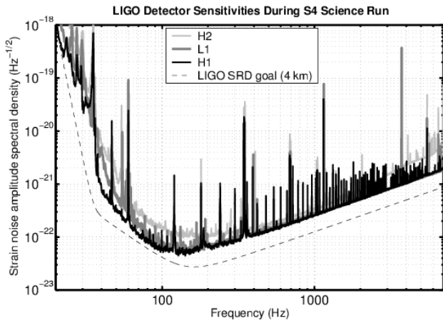
FIG. 1: Median amplitude strain noise spectral densities from the three LIGO interferometers during the S4 run, along with the Initial LIGO design sensitivity goal.
