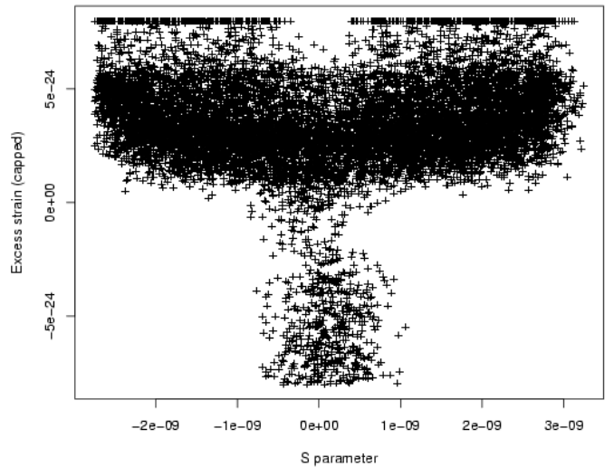
FIG. 21: “Excess” (upper limit minus injected) strain plotted vs S parameter defined in text, where values greater than 8 \times 10^{-24} have been “capped” at that ceiling value.
