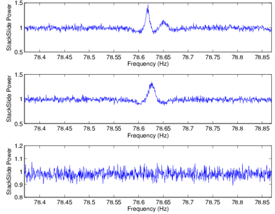
FIG. 26: The StackSlide Power vs. frequency for H1 (top), L1 (middle) and H2 (bottom) using the sky position and the \dot{f} value of the template that gives the outlier in H1 for outlier number 1 given in Table IX.
