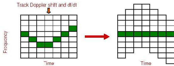
FIG. 2: An illustration of the discrete frequency bins of the Short Fourier Transform (SFTs) of the data are shown vertically, with the discrete start times of the SFTs shown horizontally. The dark pixels represent a signal in the data. Its frequency changes with time due to Doppler shifts and intrinsic evolution of the source. By sliding the frequency bins, the power from a source can be lined up and summed after appropriate weighting or transformation. This is, in essence, the starting point for all of the semi-coherent search methods presented here, though the actual implementations differ significantly.
