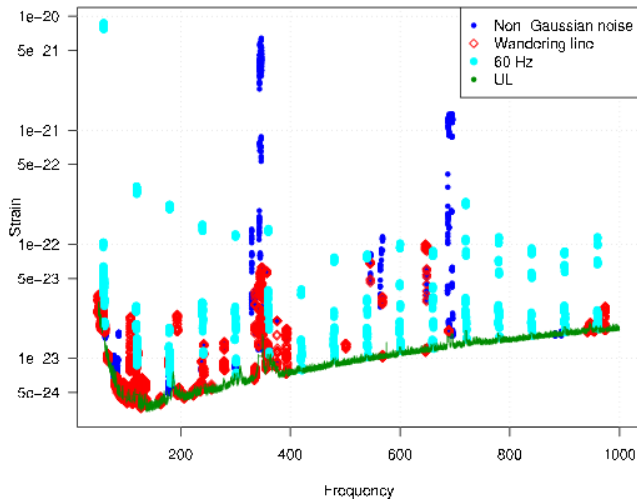
FIG. 35: PowerFlux limits on linearly polarized CW radiation amplitude for the H1 data from the S4 run. Bands flagged as non-Gaussian (instrumental artifacts) or near 60-Hz harmonics, and for which derived upper limits are unreliable, are indicated by color. Diamonds indicate bands for which wandering instrumental lines (or very strong injected signals) lead to degraded upper limits.
