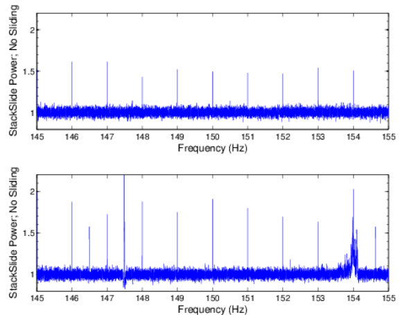
FIG. 4: The StackSlide Power for the 145 – 155 Hz band with no sliding. Harmonics of 1 Hz instrumental lines are clearly seen in H1 (top) and L1 (bottom). These lines are removed from the data by the StackSlide and Hough searches using the method described in the text, while PowerFlux search tracks these lines and avoids them when setting upper limits.
