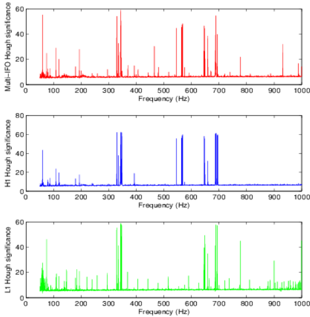
FIG. 30: Hough significance of the outliers that have survived the coincidence analysis without considering the bands contaminated with 60 Hz harmonics or the violin modes. Points are plotted only for multi-interferometer templates with significance greater than 7 and for single-interferometer templates with significance greater than 6.6.
