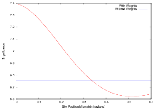
FIG. 7: The improvement in the significance as a function of the mismatch in the sky-position. A signal is injected in fake noise at \alpha = \delta = 0 and the weights are calculated at \alpha = \delta = \delta\theta . The curve is the observed significance as a function of \delta\theta while the horizontal line is the observed significance when no weights are used. See main text for more details.
