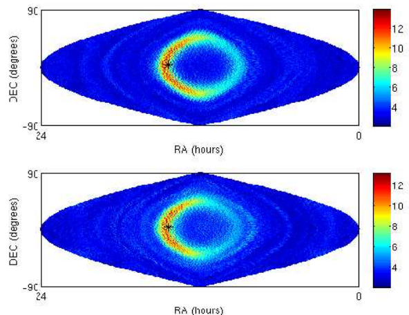
FIG. 16: Detection of hardware injected Pulsar 2 by the StackSlide code in the H1 (top) and L1 (bottom) data.
